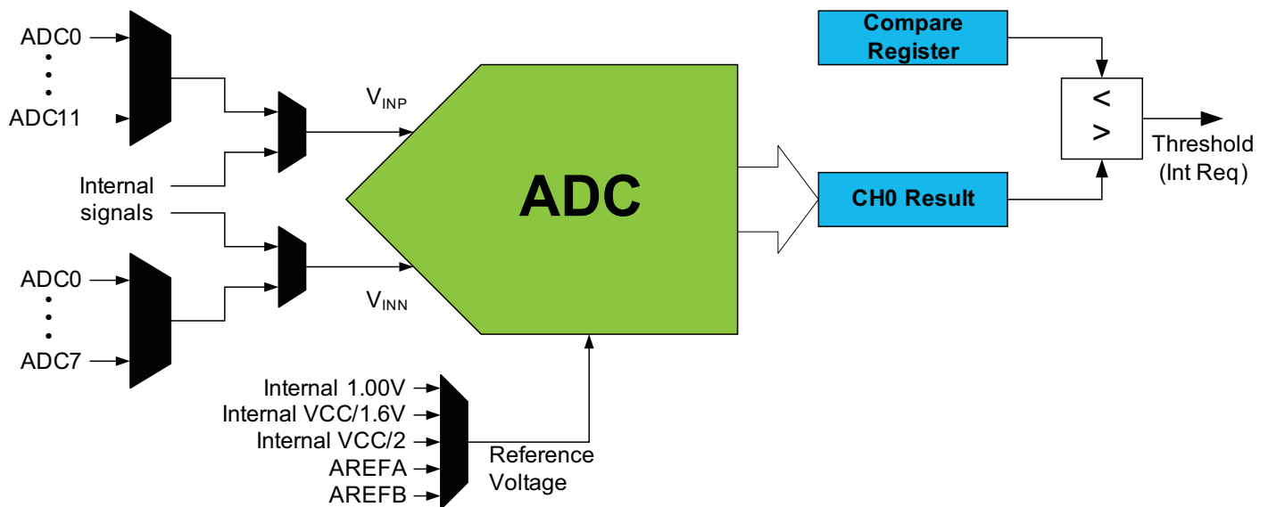
Figure 25-1. ADC overview.
