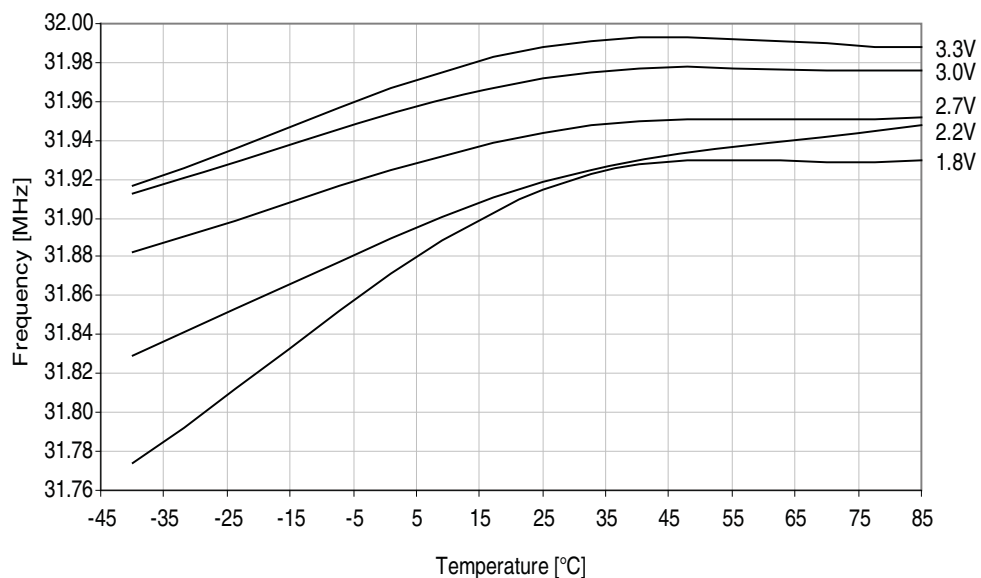
Figure 33-59. 32MHz internal oscillator frequency vs. temperature.
