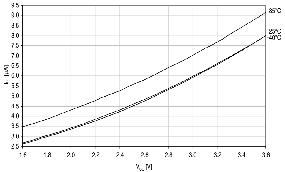
Figure 33-19. Standby supply current vs. V_{CC} . Standby, f_{SYS} = 1\text{MHz} .
